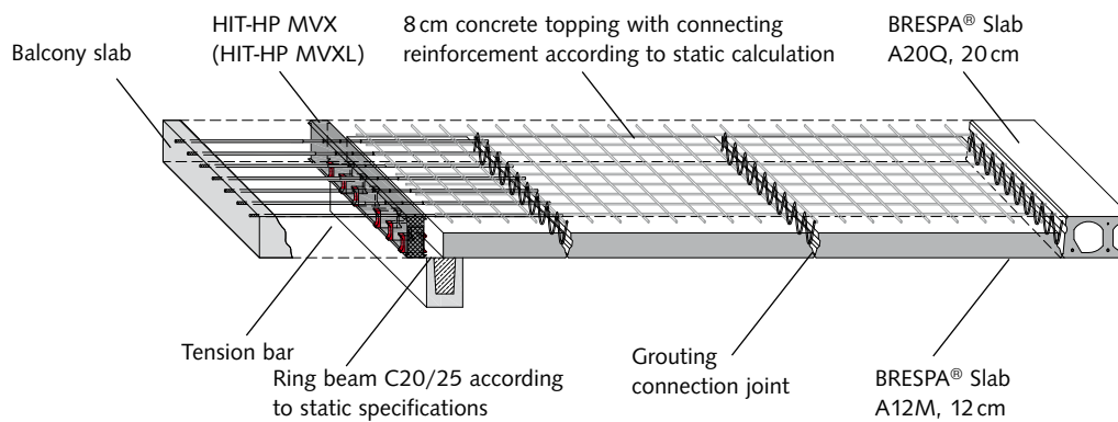
Fig.: Balcony connection using HALFEN HIT-Insulated connection and concrete topping to BRESPA® solid slab element
