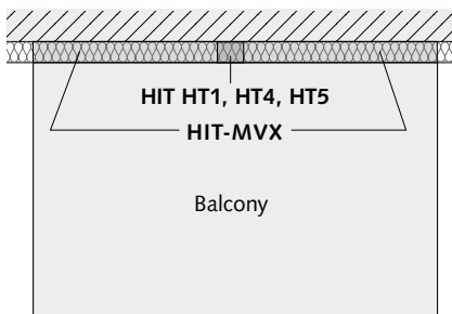
Application: Cantilevered balcony
