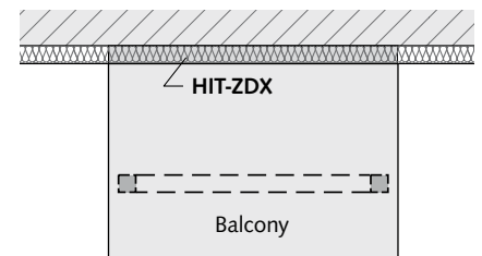
Application: Simply supported balcony on columns
