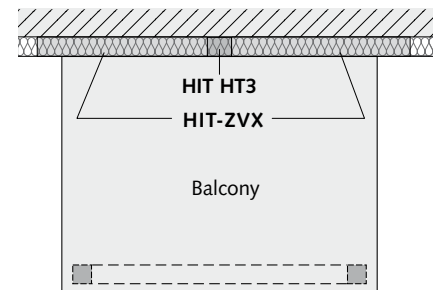
Application: Simply supported balcony on columns
